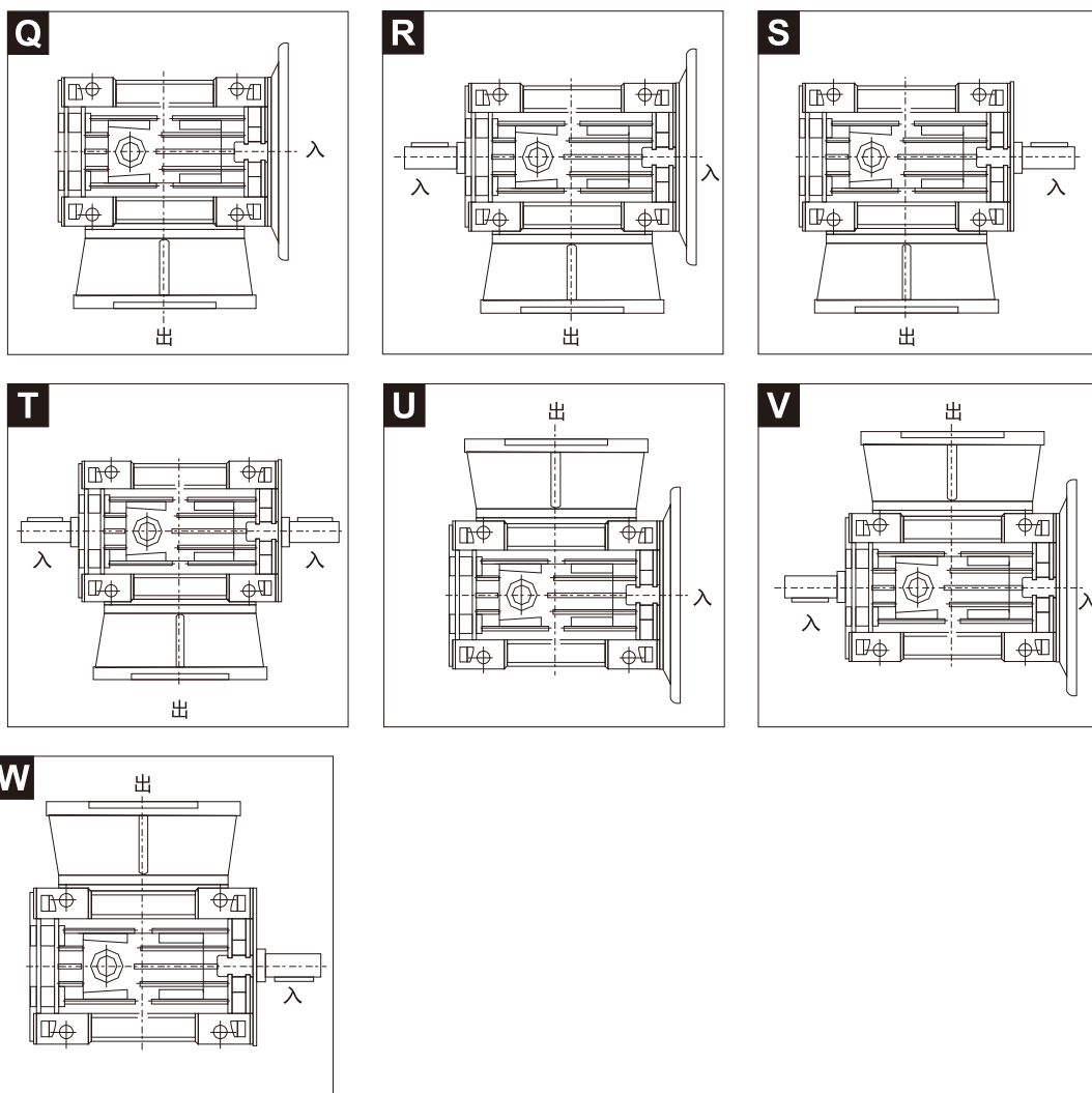
Directions of input shaft & output flange
